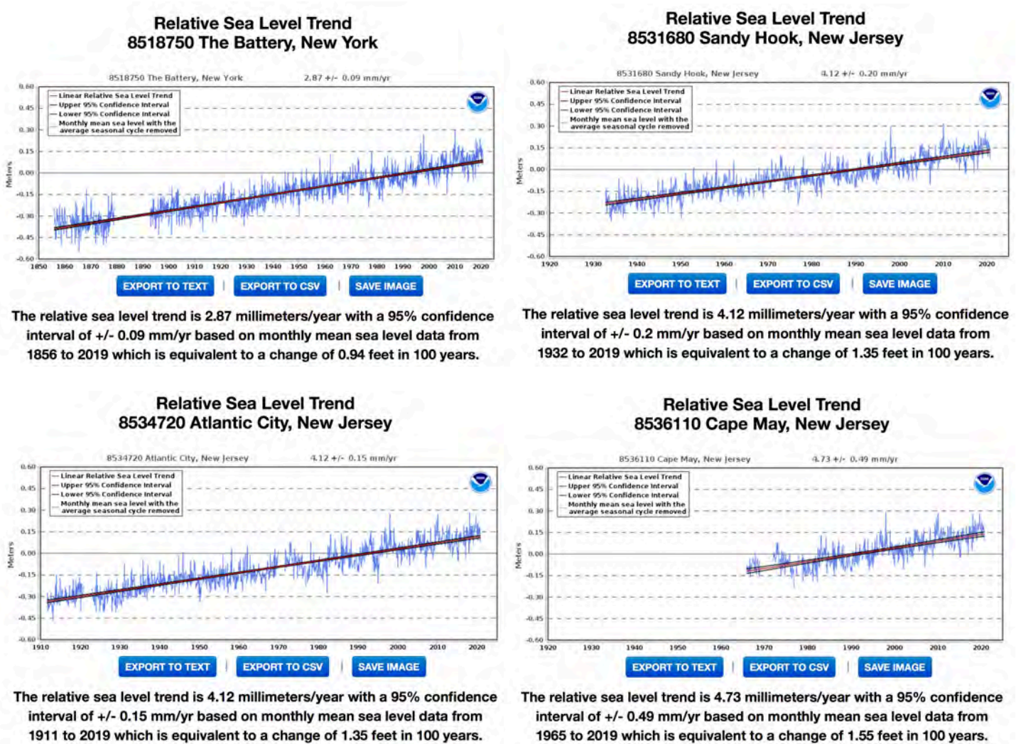
Figure 4.1: Historic monthly relative sea level values and trends for NJ locations of Sandy Hook (upper right), Atlantic City (lower left) and Cape May (lower right) as well as The Battery in New York (upper left). All plots can be reproduced at https://tidesandcurrents.noaa.gov/map/index.html?region=New%20Jersey
